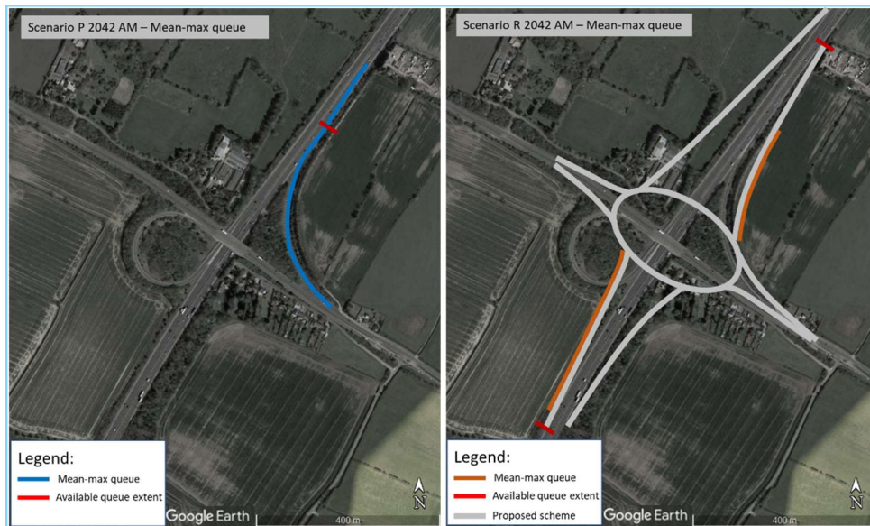
Figure 25 – Mean-max queue M5 off-slips 2042 AM Peak
